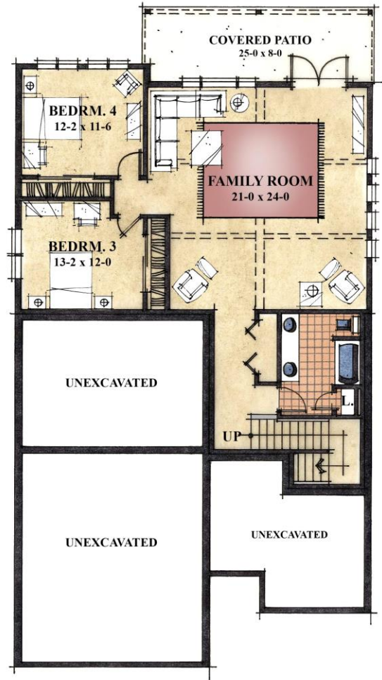
Lower Level
