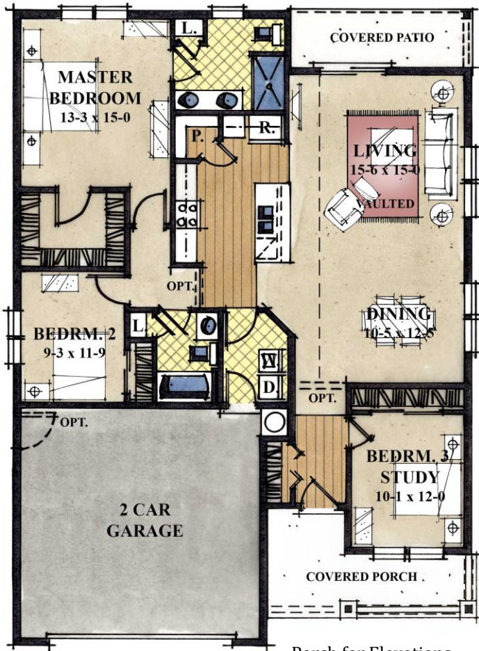
Porch for Elevations 2 & 4
