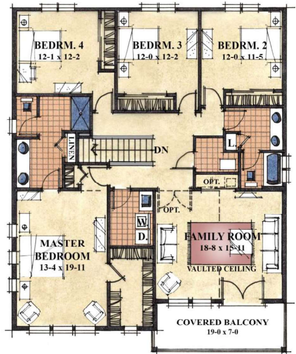
Upper Level
