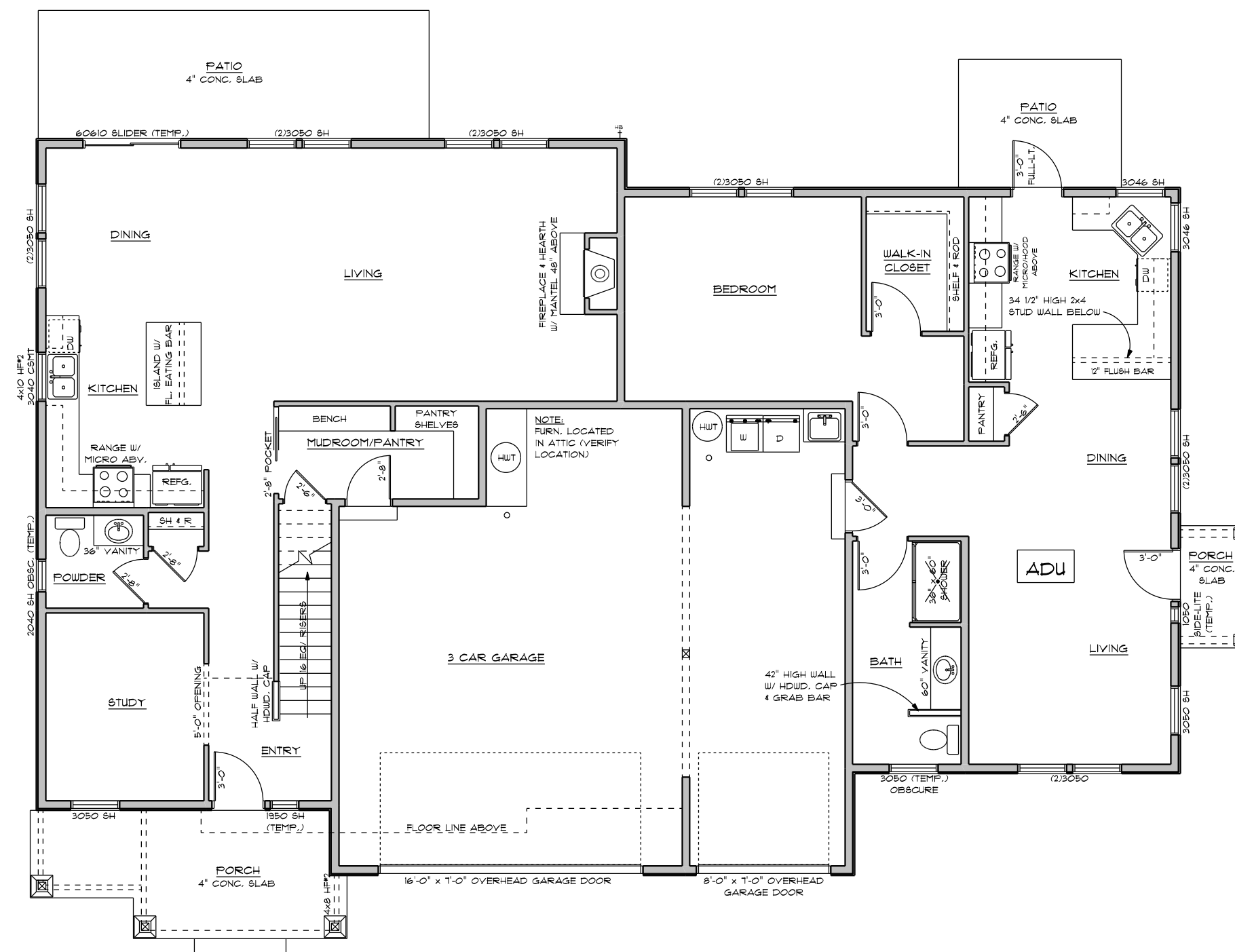
MAIN FLOOR PLAN HOUSE: 1288 SQ. FT. ADU: 897 SQ. FT.
